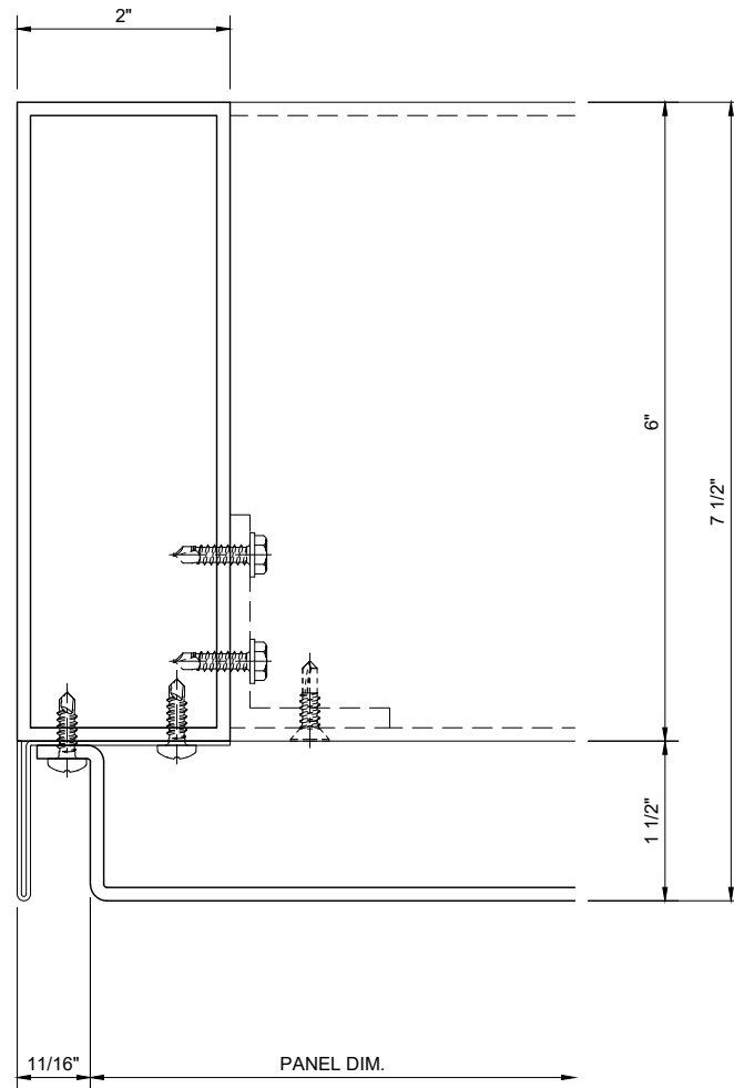
JAMB PLAN DETAIL SCALE: 6" = 1'-0"
