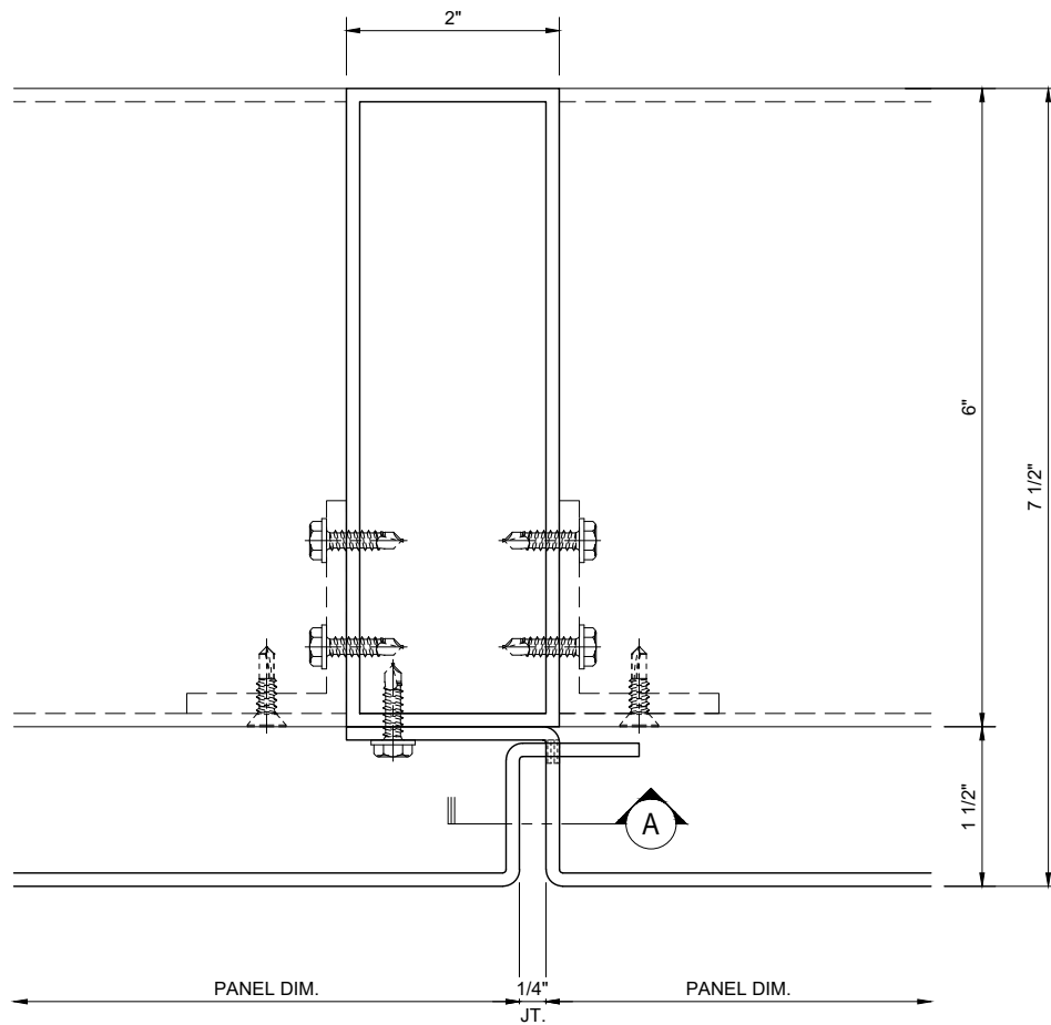
INTERMEDIATE PLAN DETAIL SCALE: 6" = 1'-0"
