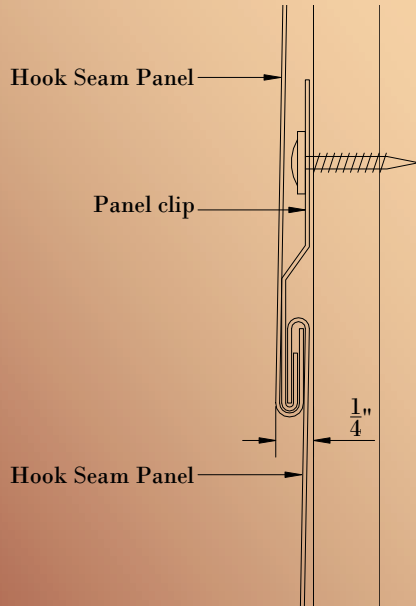
Panel Profile
